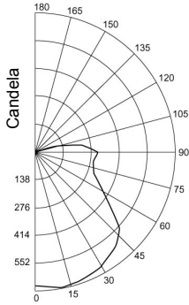
MTWA70MH* 70W Medium Base MH NEMA Type: 7x7 Lumens - 9000 * Insert Top Style
