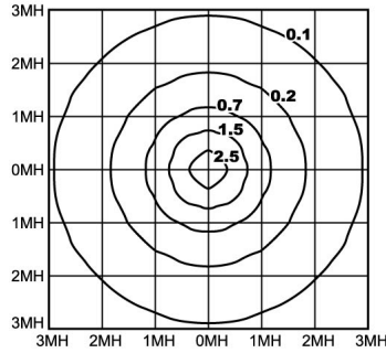
MTWA70MH* 70W Medium Base MH Lumens - 9000 * Insert Top Style Mounting Height = 15'
