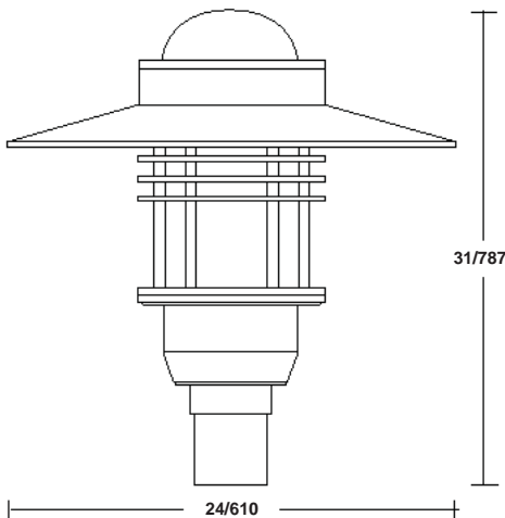
Fully Shielded, IESNA Full Cutoff 150W maximum, Horizontal Lamp Dimensions include Dome Top Option Hub fits onto 2-3/8" tenon
