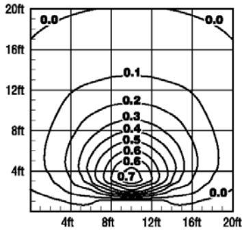
SLS18CFLHCG 18W Compact Fluorescent 6' Mounting Height
