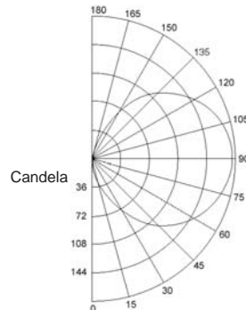
SLS18CFLOF 18W Compact Fluorescent NEMA Type: 7x7 Lumens - 1200
