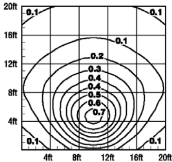
SLS18CFL3SG 18W Compact Fluorescent 6' Mounting Height
