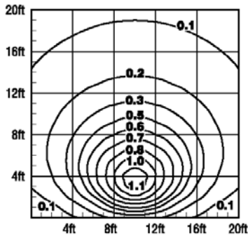
SLS18CFLSCG 18W Compact Fluorescent 6' Mounting Height
