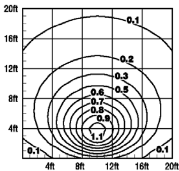
SLS18CFLDCG 18W Compact Fluorescent 6' Mounting Height
