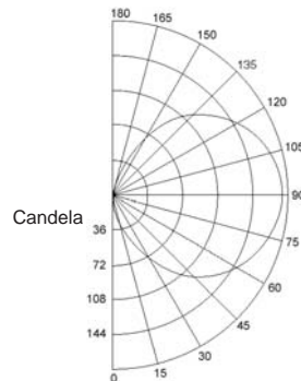
SLS18CFLSCG 18W Compact Fluorescent NEMA Type: 7x7 Lumens - 1200
