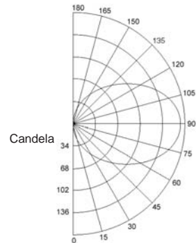
SLS18CFL3SG 18W Compact Fluorescent NEMA Type: 7x7 Lumens - 1200
