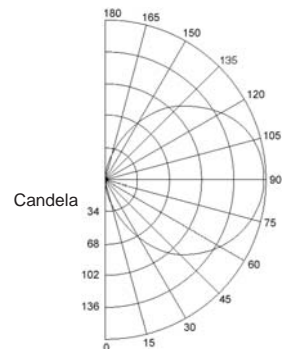
SLS18CFLDCG 18W Compact Fluorescent NEMA Type: 7x7 Lumens - 1200
