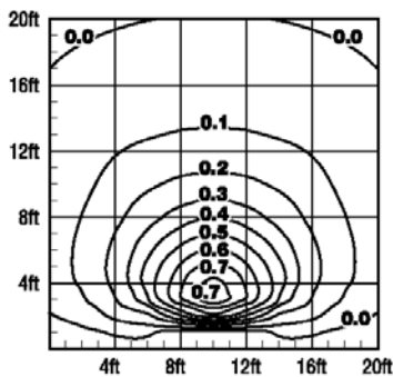
SLS18CFLHC 18W Compact Fluorescent 6' Mounting Height
