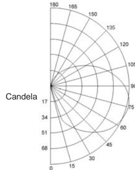
SLS18CFLHCG 18W Compact Fluorescent NEMA Type: 7x6 Lumens - 1200
