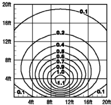
SLS18CFLOF 18W Compact Fluorescent 6' Mounting Height
