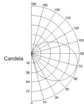
SLS18CFLHC 18W Compact Fluorescent NEMA Type: 7x6 Lumens - 1200
